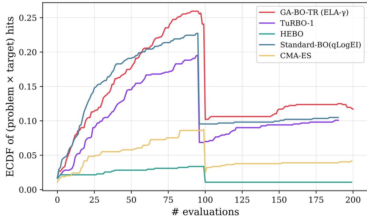
BBOB-24 ECDF — fraction of targets reached
